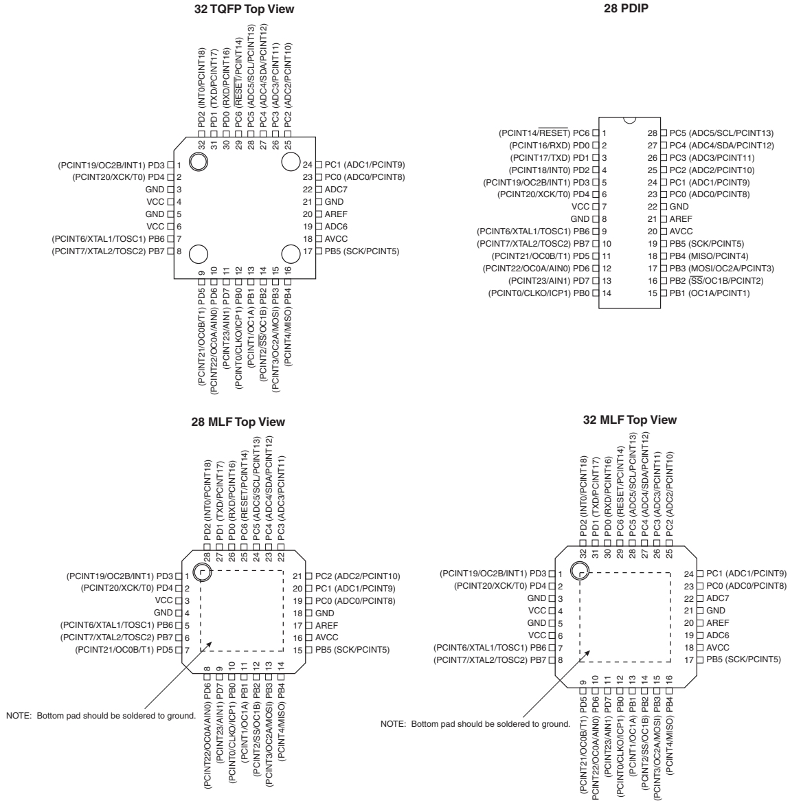
Figure 1-1. Pinout ATmega48A/48PA/88A/88PA/168A/168PA/328/328P
